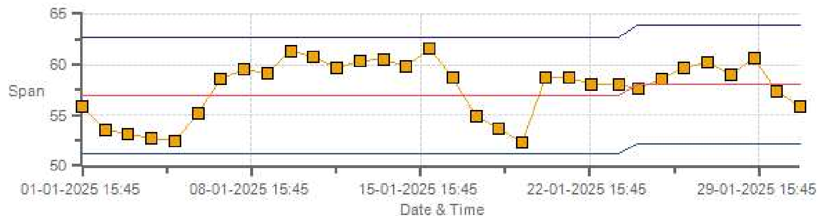
TRS[ppb] Calibration: PRAMP 986-C Monthly: 01-2025 Type: SpanAndZero - Span
