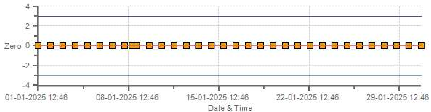
THC55[ppm] Calibration: PRAMP 842-B Monthly: 01-2025 Type: SpanAndZero - Zero
