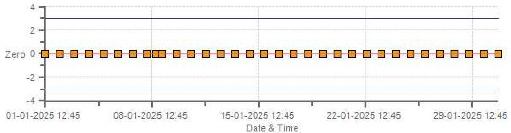
CH4[ppm] Calibration: PRAMP 842-B Monthly: 01-2025 Type: SpanAndZero - Zero
