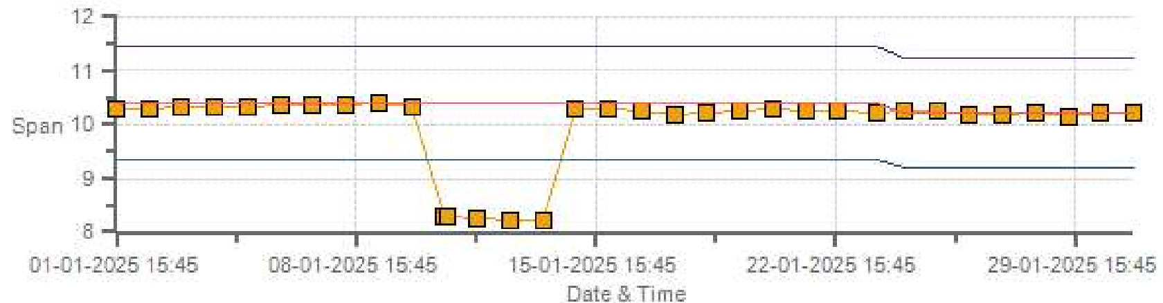
CH4[ppm] Calibration: PRAMP 986-C Monthly: 01-2025 Type: SpanAndZero - Span
