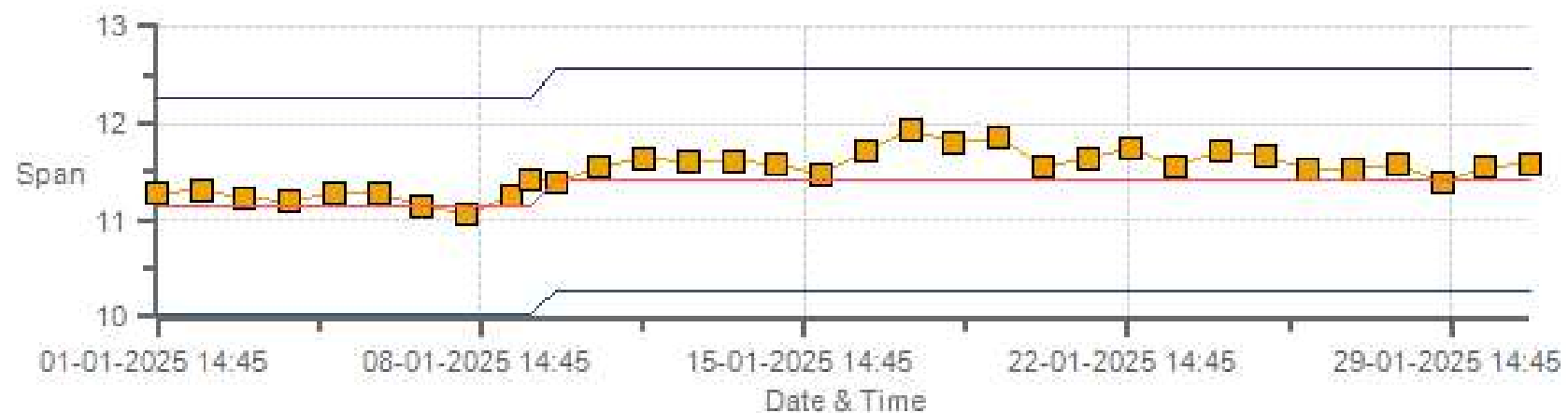
NMHC[ppm] Calibration: PRAMP RENO-B Monthly: 01-2025 Type: SpanAndZero - Span
