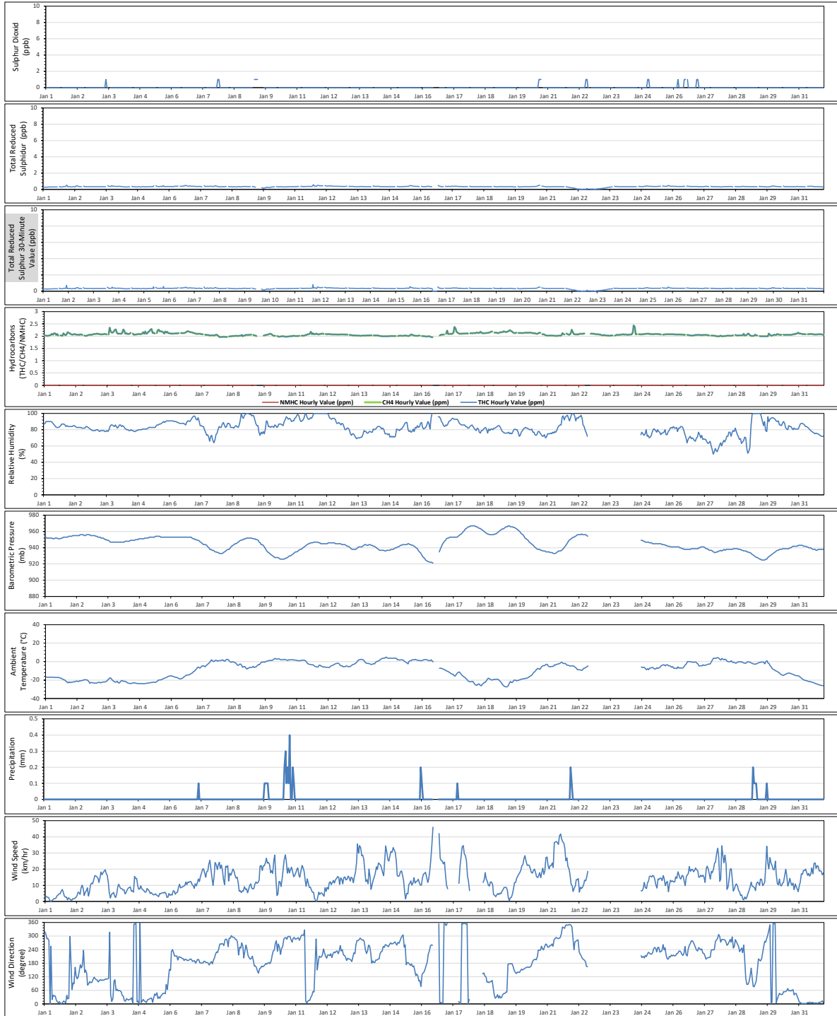
Timeseries Chart of Hourly Average for the month of Jan 2025 - Reno-B Station
