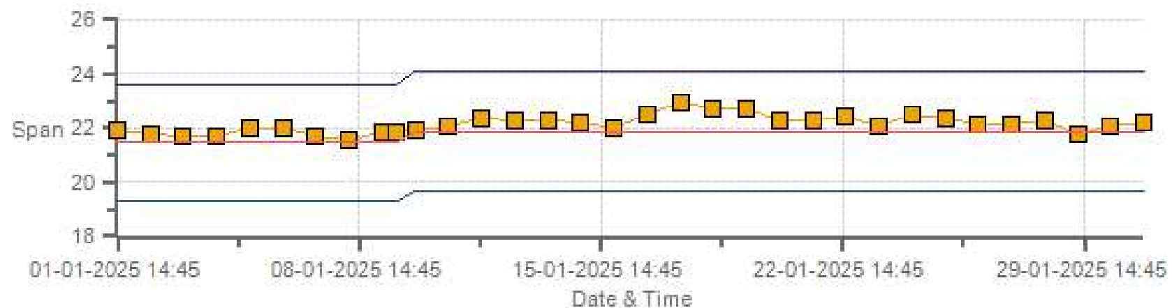
THC55[ppm] Calibration: PRAMP RENO-B Monthly: 01-2025 Type: SpanAndZero - Span
