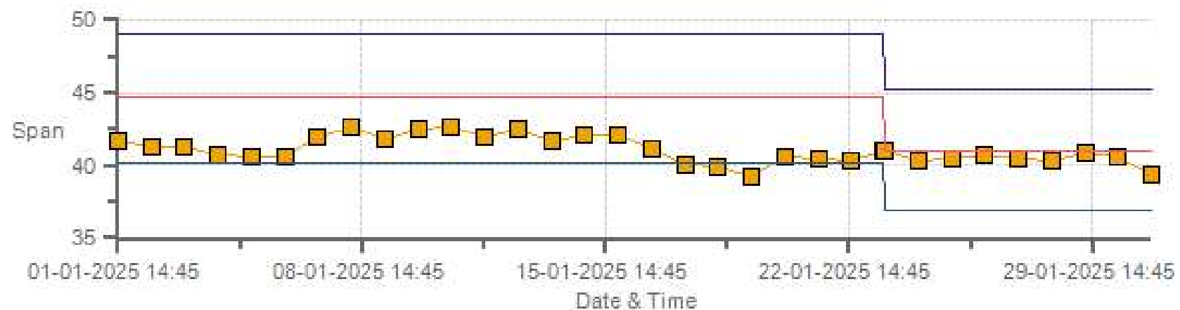
TRS[ppb] Calibration: Peace River Complex [PRC] Monthly: 01-2025 Type: SpanAndZero - Span
