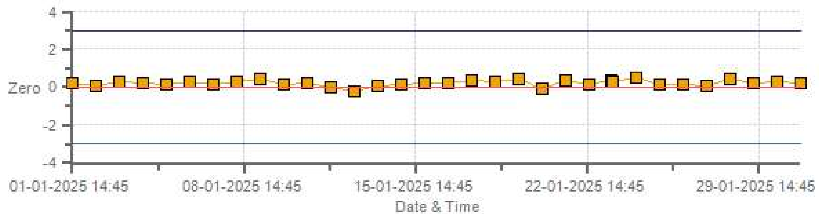
SO 2 [ppb] Calibration: Peace River Complex [PRC] Monthly: 01-2025 Type: SpanAndZero - Zero
