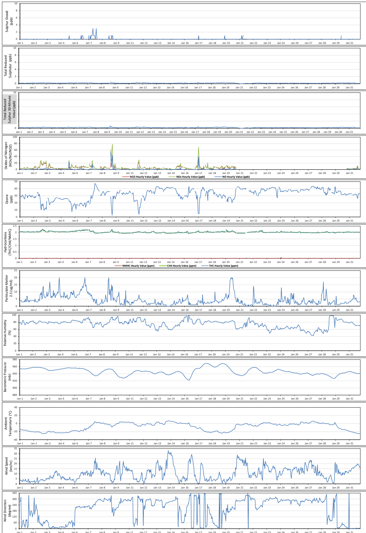
Timeseries Chart of Hourly Average for the month of Jan 2025 - AQHI - Grimshaw Station
