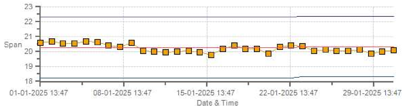
THC55[ppm] Calibration: AQHI Grimshaw Monthly: 01-2025 Type: SpanAndZero - Span
