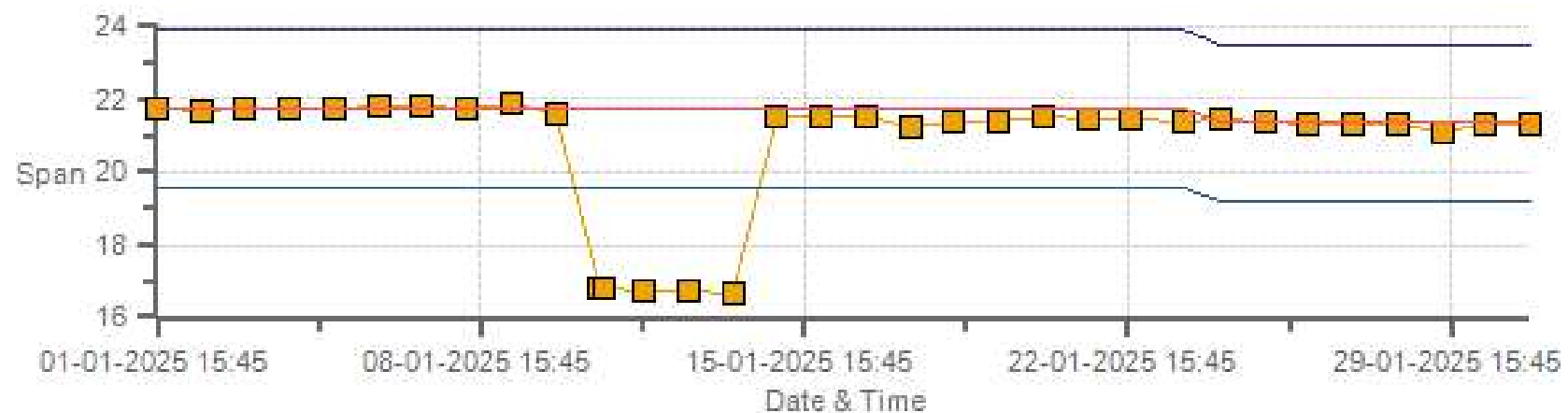
THC55[ppm] Calibration: PRAMP 986-C Monthly: 01-2025 Type: SpanAndZero - Span
