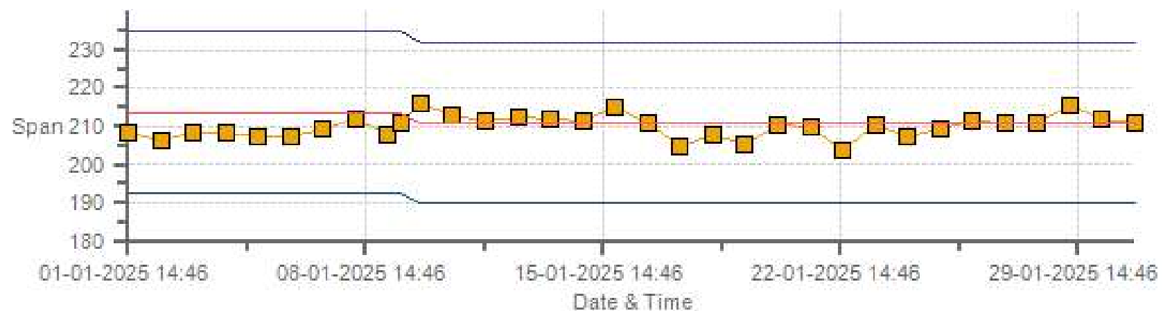
SO2[ppb] Calibration: PRAMP RENO-B Monthly: 01-2025 Type: SpanAndZero - Span
