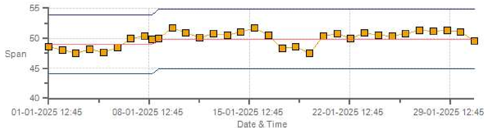
TRS[ppb] Calibration: PRAMP 842-B Monthly: 01-2025 Type: SpanAndZero - Span
