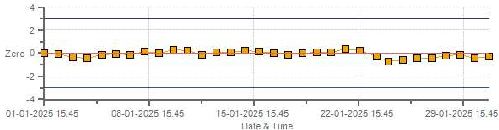
SO2[ppb] Calibration: PRAMP 986-C Monthly: 01-2025 Type: SpanAndZero - Zero
