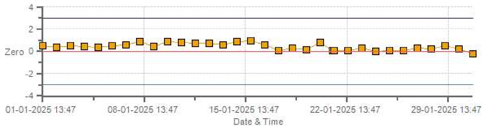
SO2[ppb] Calibration: AQHI Grimshaw Monthly: 01-2025 Type: SpanAndZero - Zero
