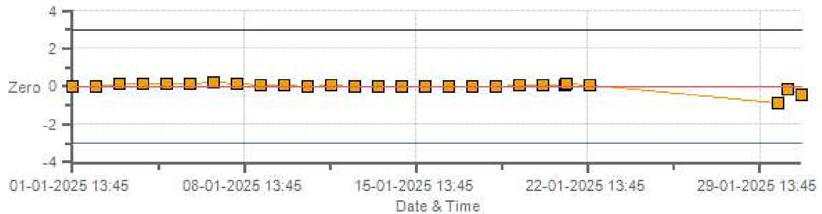
NO2[ppb] Calibration: AQHI Grimshaw Monthly: 01-2025 Type: SpanAndZero - Zero
