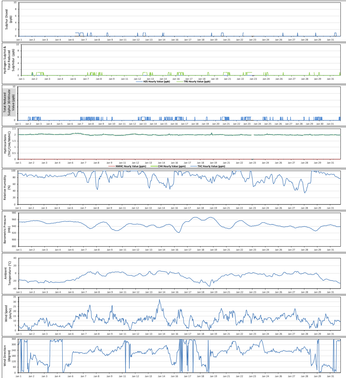
Timeseries Chart of Hourly Average for the month of Jan 2025 - Peace River Complex (PRC) Station
