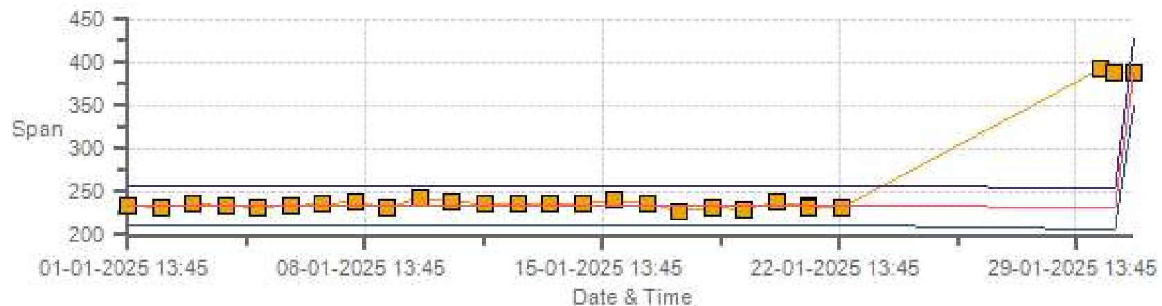
NOX[ppb] Calibration: AQHI Grimshaw Monthly: 01-2025 Type: SpanAndZero - Span
