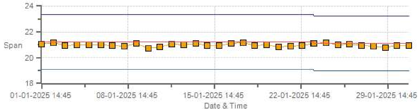
THC55[ppm] Calibration: Peace River Complex [PRC] Monthly: 01-2025 Type: SpanAndZero - Span
