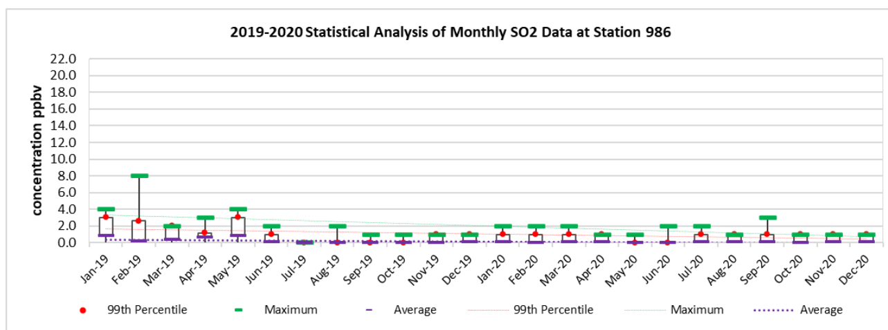
Figure 23: Sulphur Dioxide Data and Trends at Station 986
