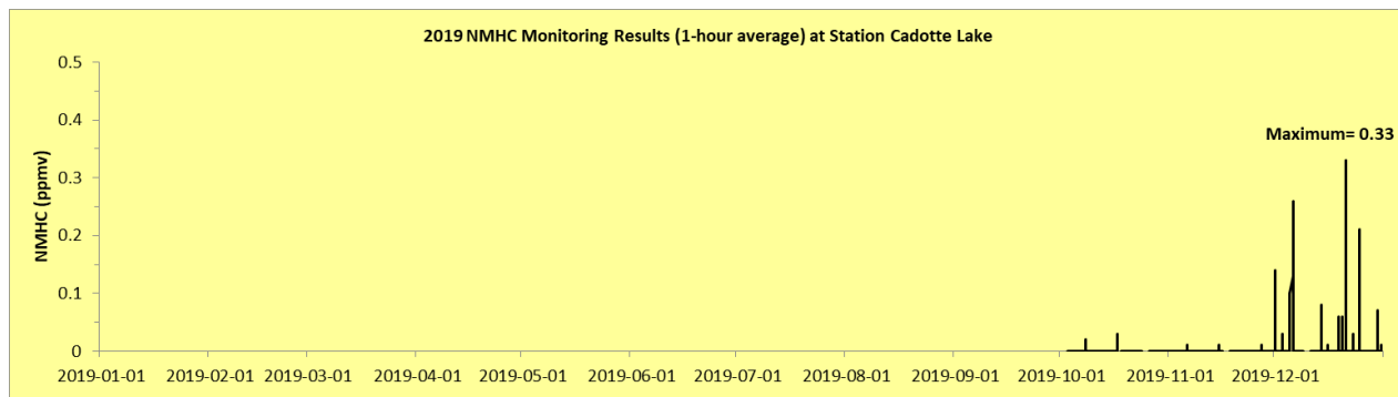
Figure 5: Hourly Monitored Non-Methane Hydrocarbons Data
