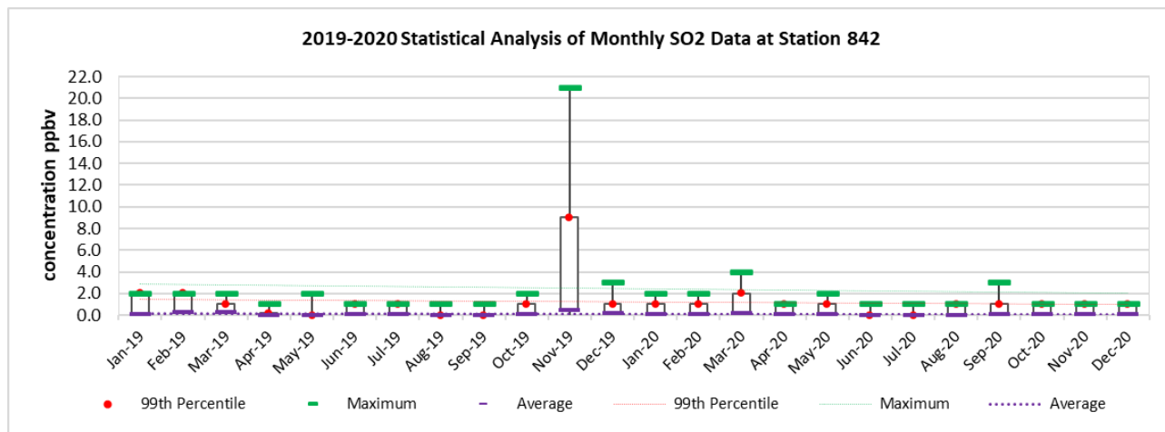
Figure 22: Sulphur Dioxide Data and Trends at Station 842
