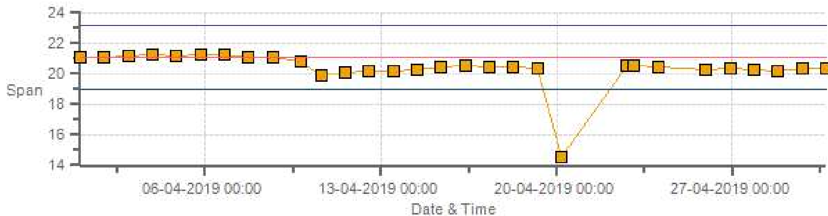
THC [ppm] Calibration: PRAMP 842 Monthly: 04-2019 Type: Span
