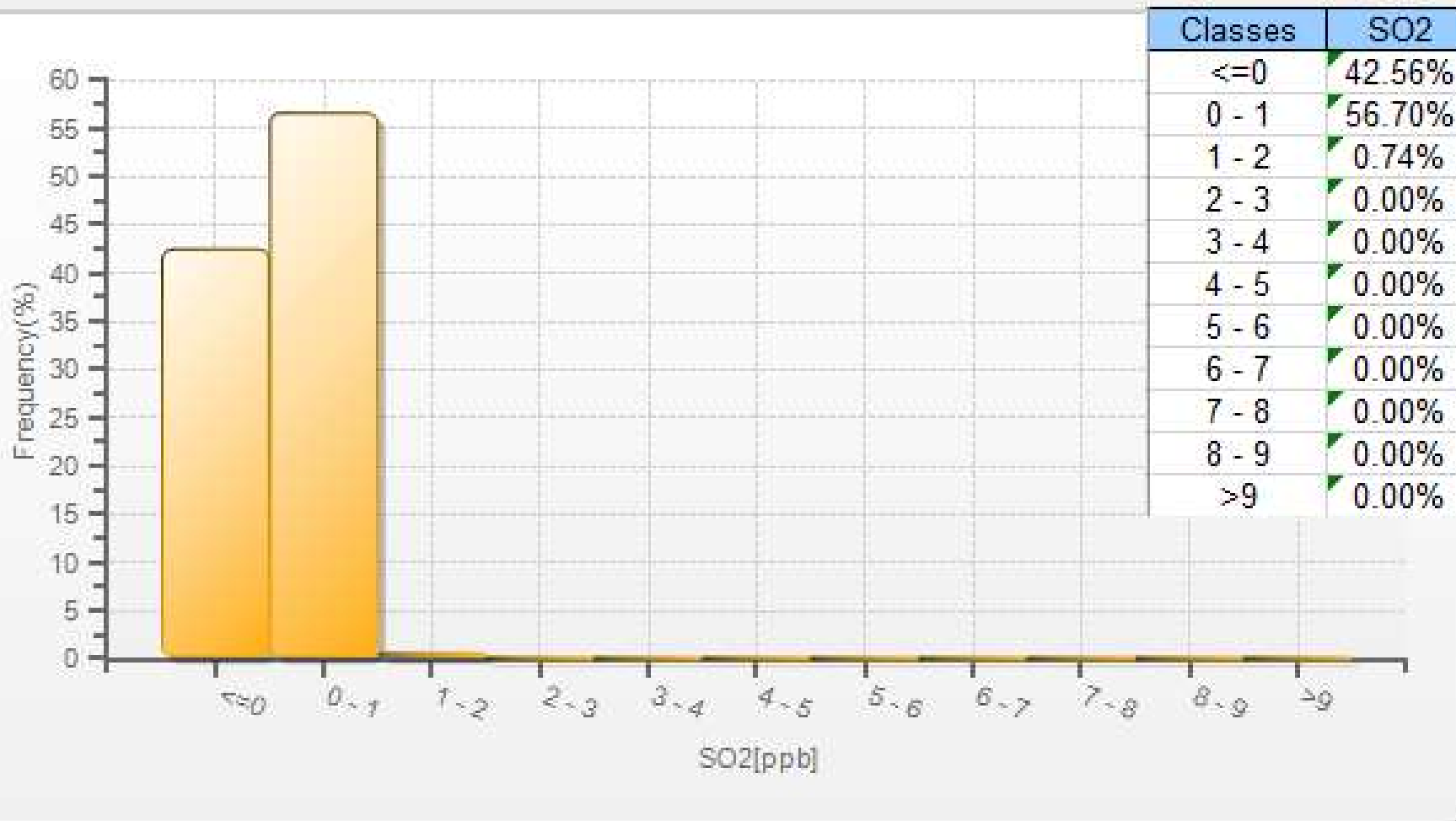
SO2[ppb] Histogram: PRAMP RENO Monthly: 04-2019 1 Hr.
