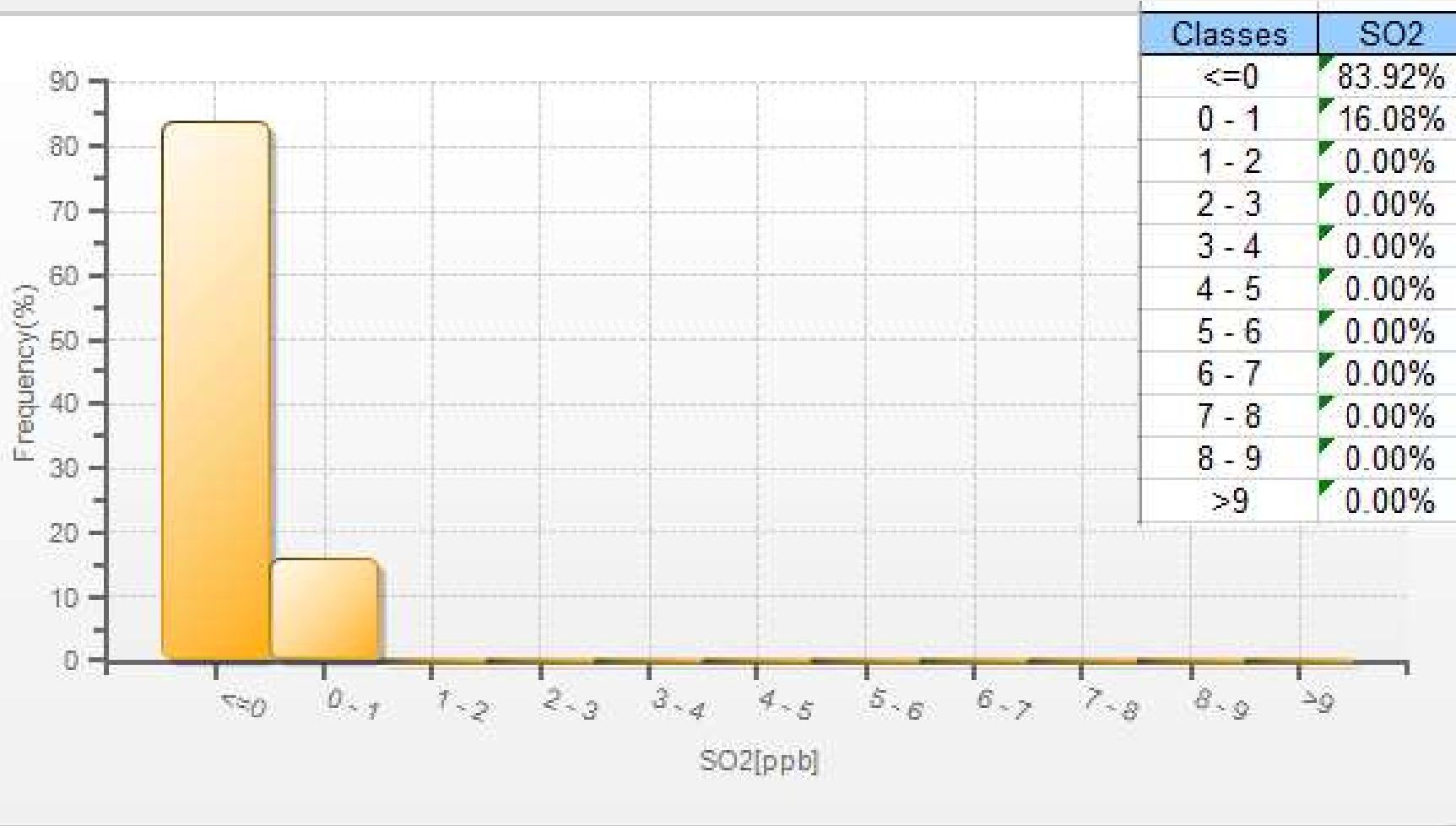
SO2[ppb] Histogram: PRAMP 842 Monthly: 04-2019 1 Hr.
