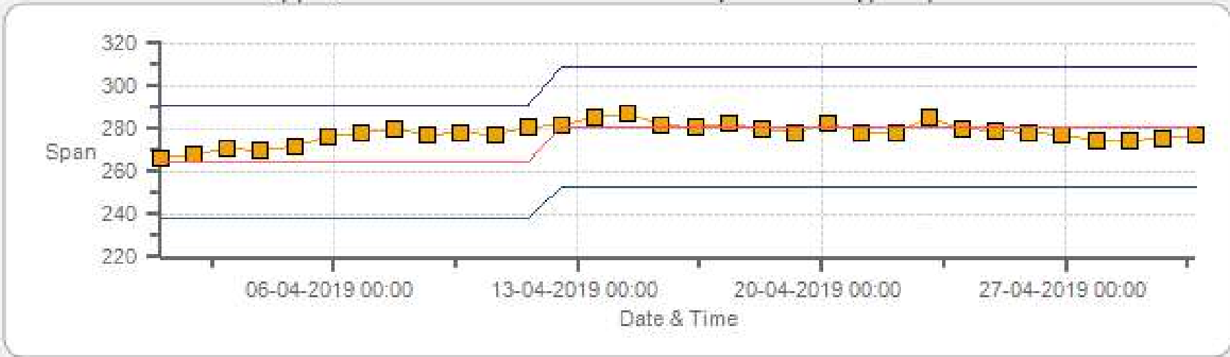
SO2 [ppb] Calibration: PRAMP 986 Monthly: 04-2019 Type: Span
